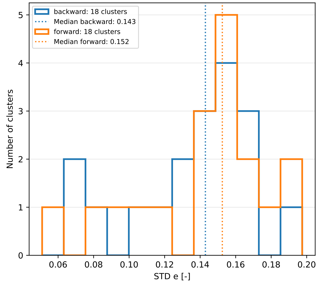
K=18 | Within-cluster STD distributions | Each cluster counts once
